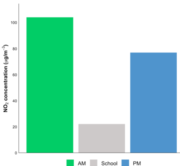
▲ Figure 7. Average \text{NO}_2 concentrations over the monitoring period across all participating schools.
