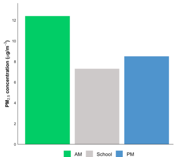
▲ Figure 8. Average \text{PM}_{2.5} concentrations over the monitoring period across all participating schools.
